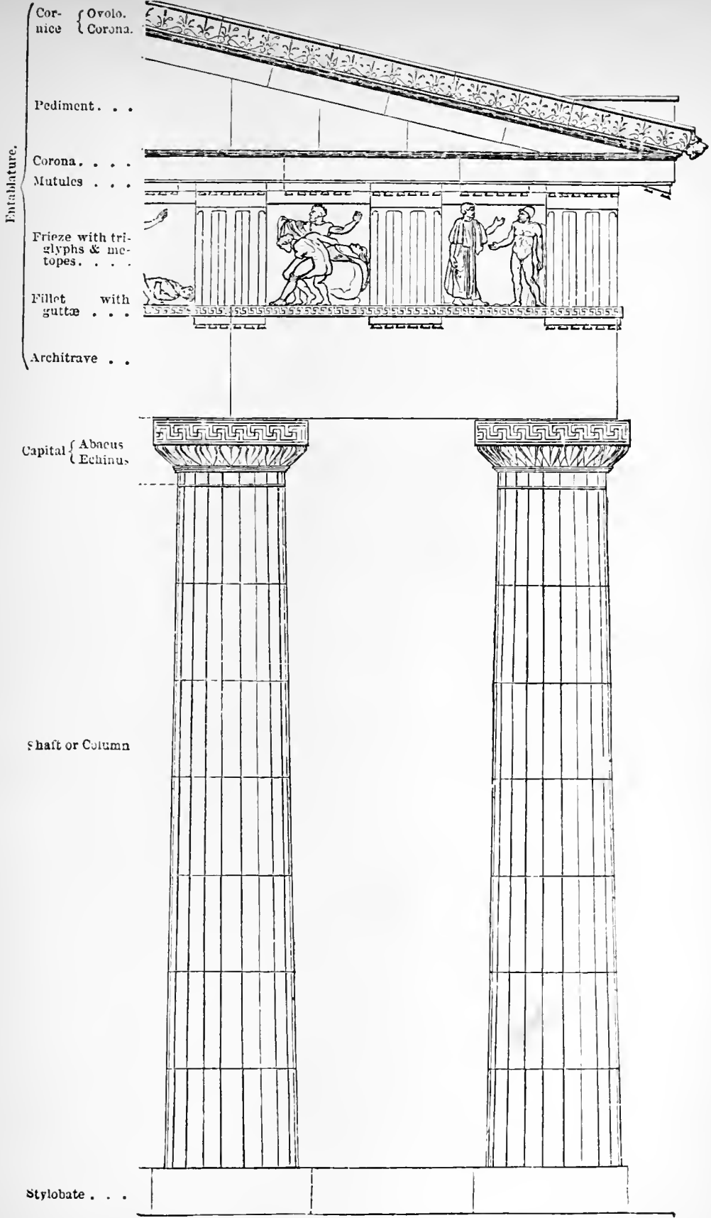
FIG. 57.—THE GREEK DORIC ORDER FROM THE THESEUM.
